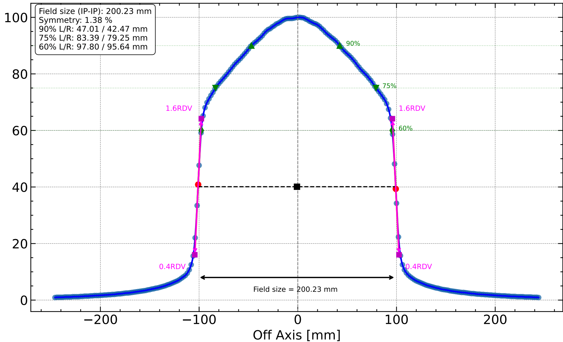
Beam Profile for 6MV FFF (20x20 cm 2 field)
